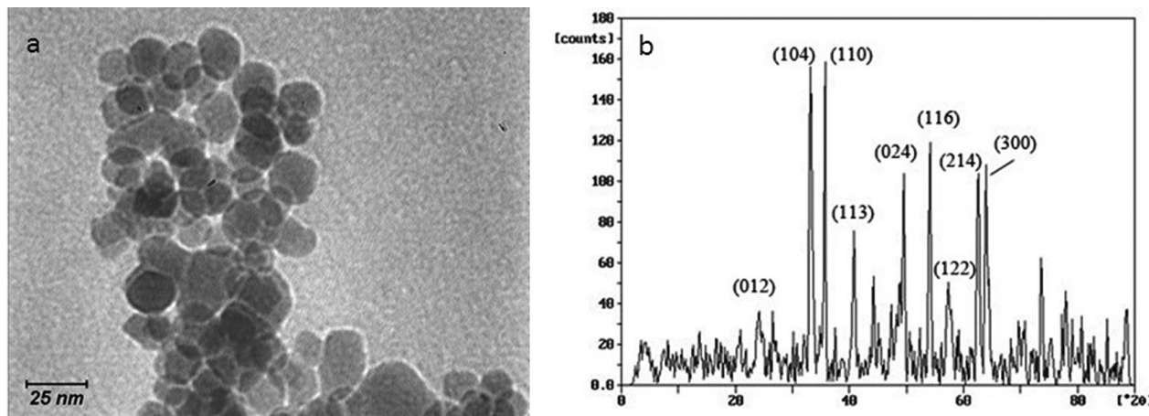
Figure 3. (a) TEM images of iron oxide nanoparticles; (b) XRD pattern of \alpha -iron oxide nanoparticles.
