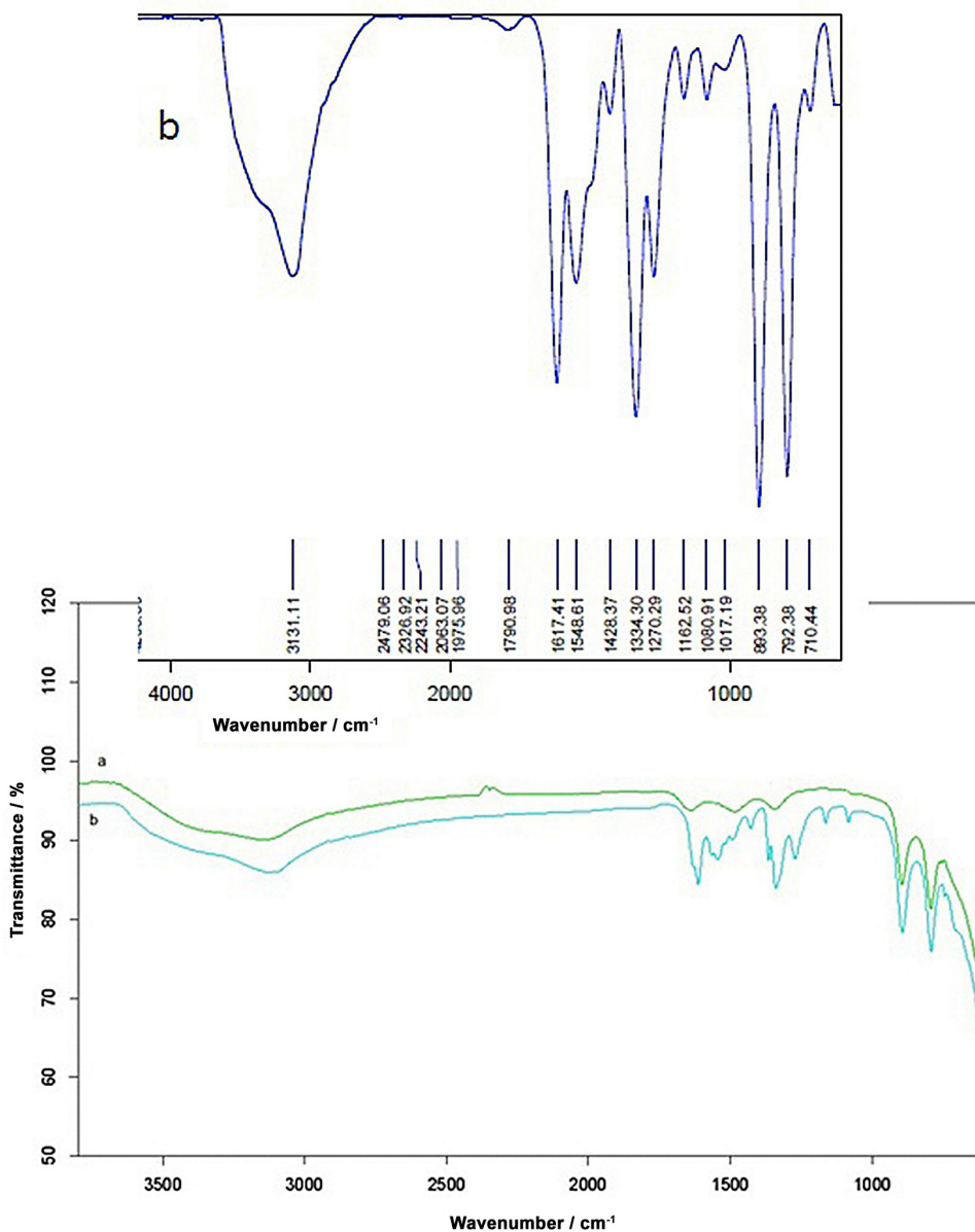
Figure 4. FTIR spectra of (a) bare iron oxide nanoparticles and (b) picric acid loaded iron oxide nanoparticles (PA-IONP). Inset: zoom of curve (b).
