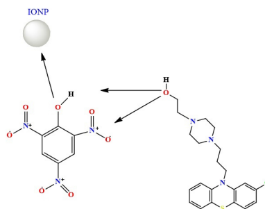
Figure 2. Positions for interaction between PPZ and PA and surface of \alpha -Fe 2 O 3 (IONP).
