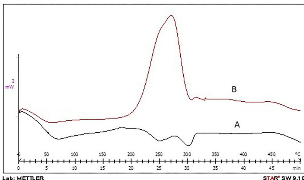
Figure 5. DSC thermogram of (A) \alpha -Fe 2 O 3 and (B) PA-IONPs.
