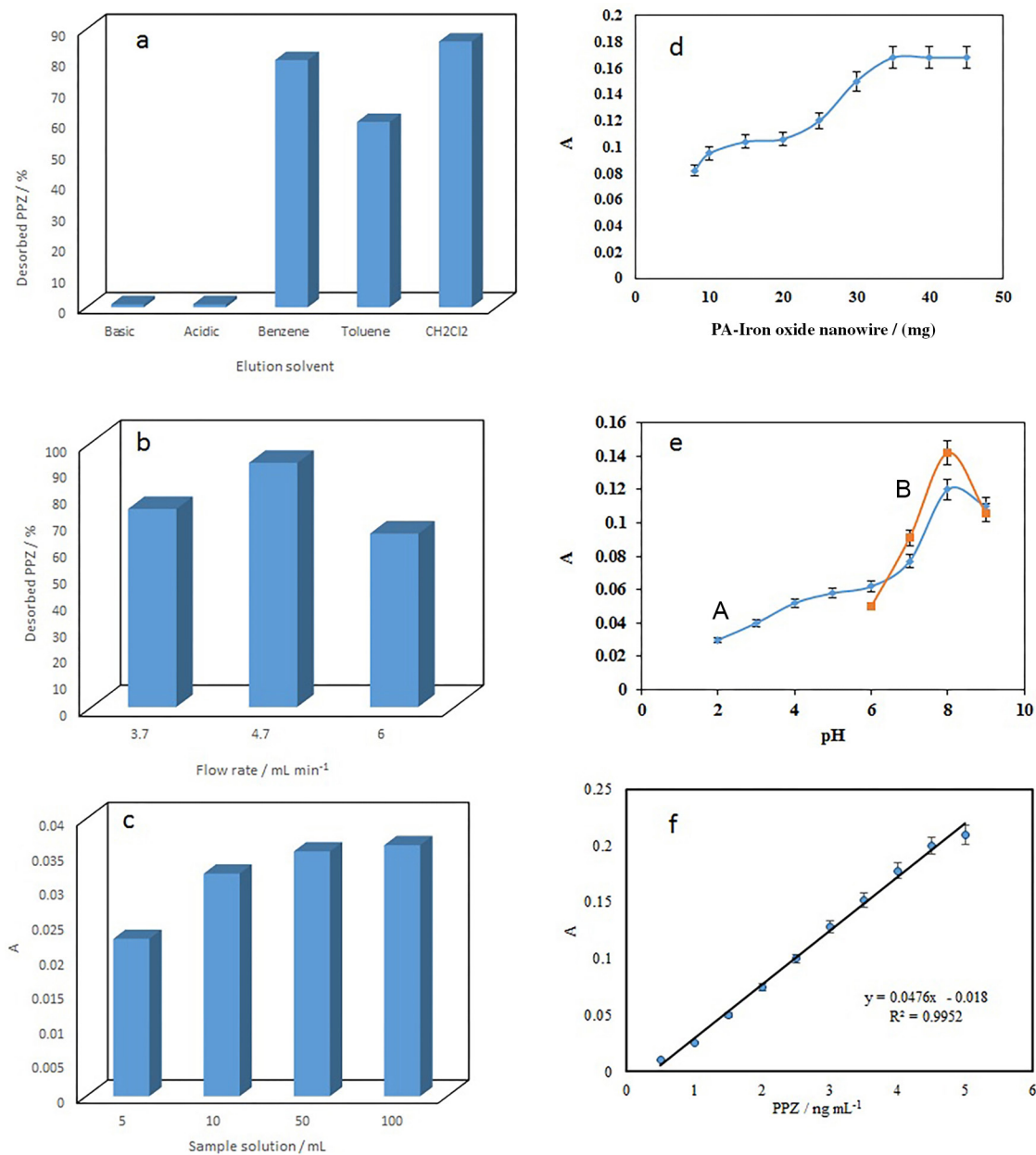
Figure 6. (a) Selection of elution solvent for PPZ desorption; (b) effect of elution solvent flow rate on PPZ desorption; (c) different volume of 1 ng mL -1 PPZ passing through PA-IONPs disc; (d) effect of PA-IONPs amount; (e) effect of pH on the pre-concentration and separation of perphenazine using PA-IONP, pH was controlled by (A) NaOH and HCl, (B) buffer solution; and (f) calibration curve for PPZ by the present method at optimum condition described in the manuscript.
